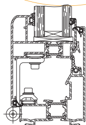
Profile with thermal bridge
