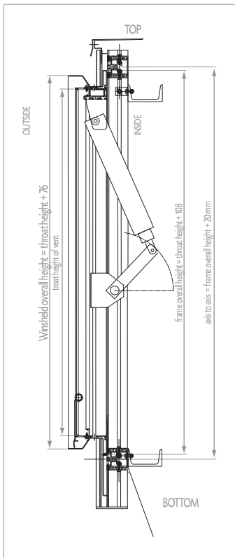
Section B-B
