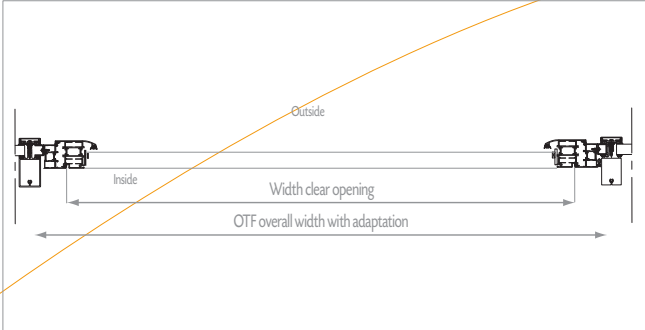
Horizontal section
