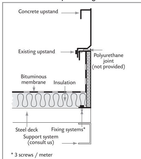
Installation on an upstand in galvanized steel
