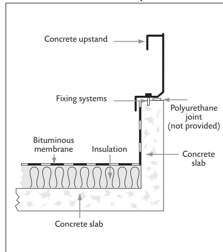
Installation on a concrete upstand
